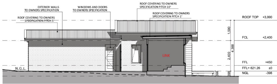
SOUTH-EAST ELEVATION
