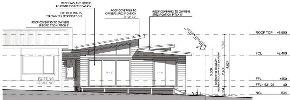
NORTH-EAST ELEVATION
