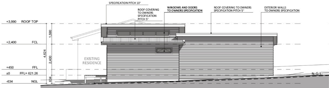
NORTH-WEST ELEVATION
