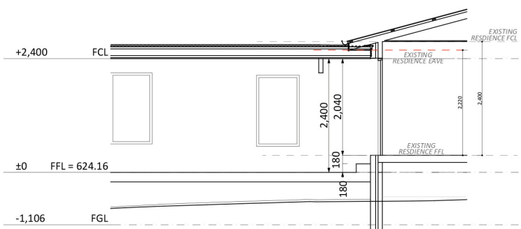
Building Section B
