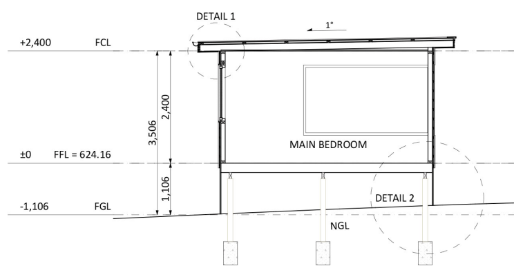
Building Section A
