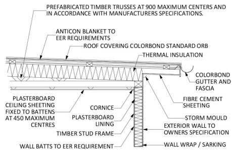
DETAIL 1 SCALE 1:20
