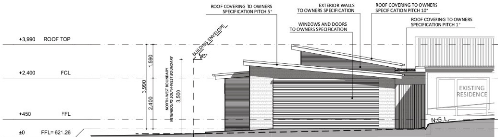
SOUTH-WEST ELEVATION
